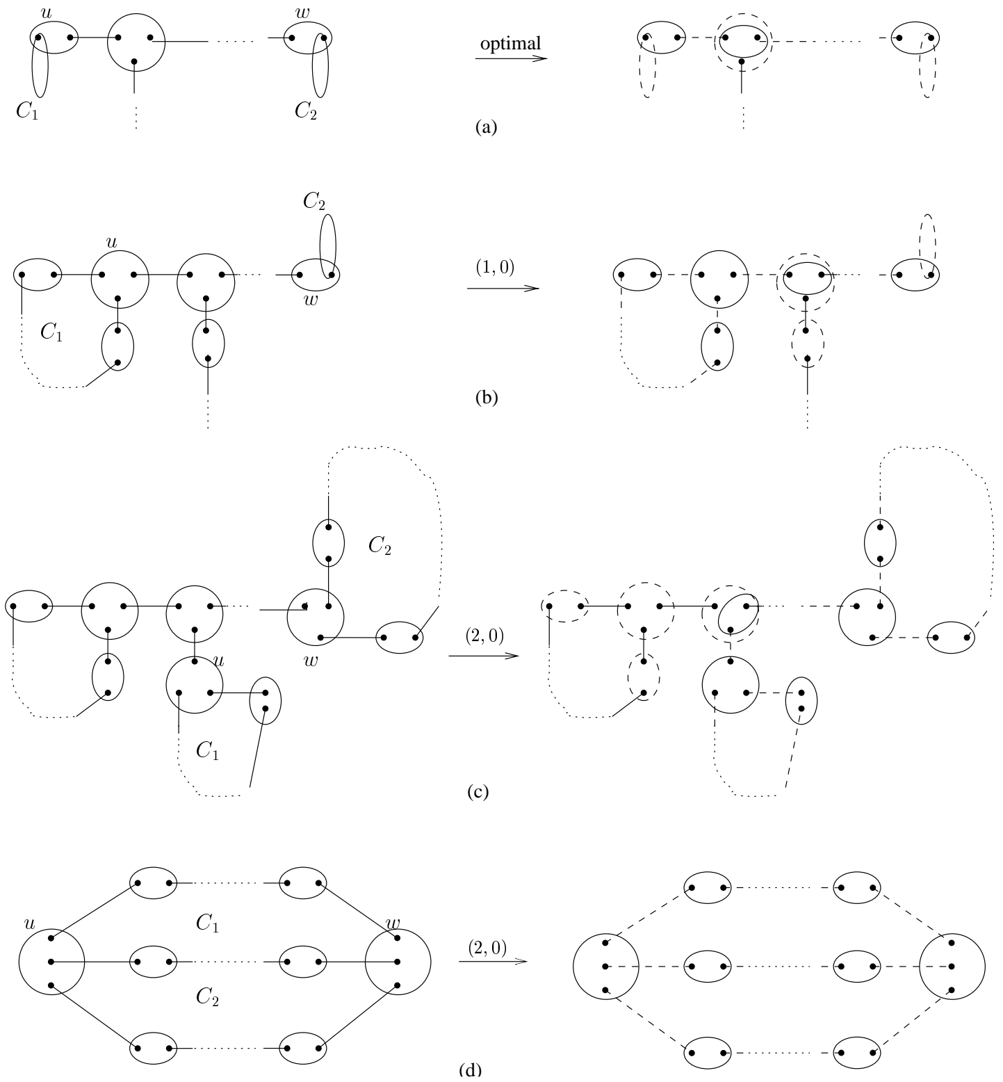
Figure 5: Examples for Lemma 3.5. (a),(b),(c) Semi-local improvement in the case when H has two disjoint cycles.(d) A (2, 0) improvement leads to a better solution when neither C_1 and C_2 are not disjoint and neither of them are 1-cycles.
