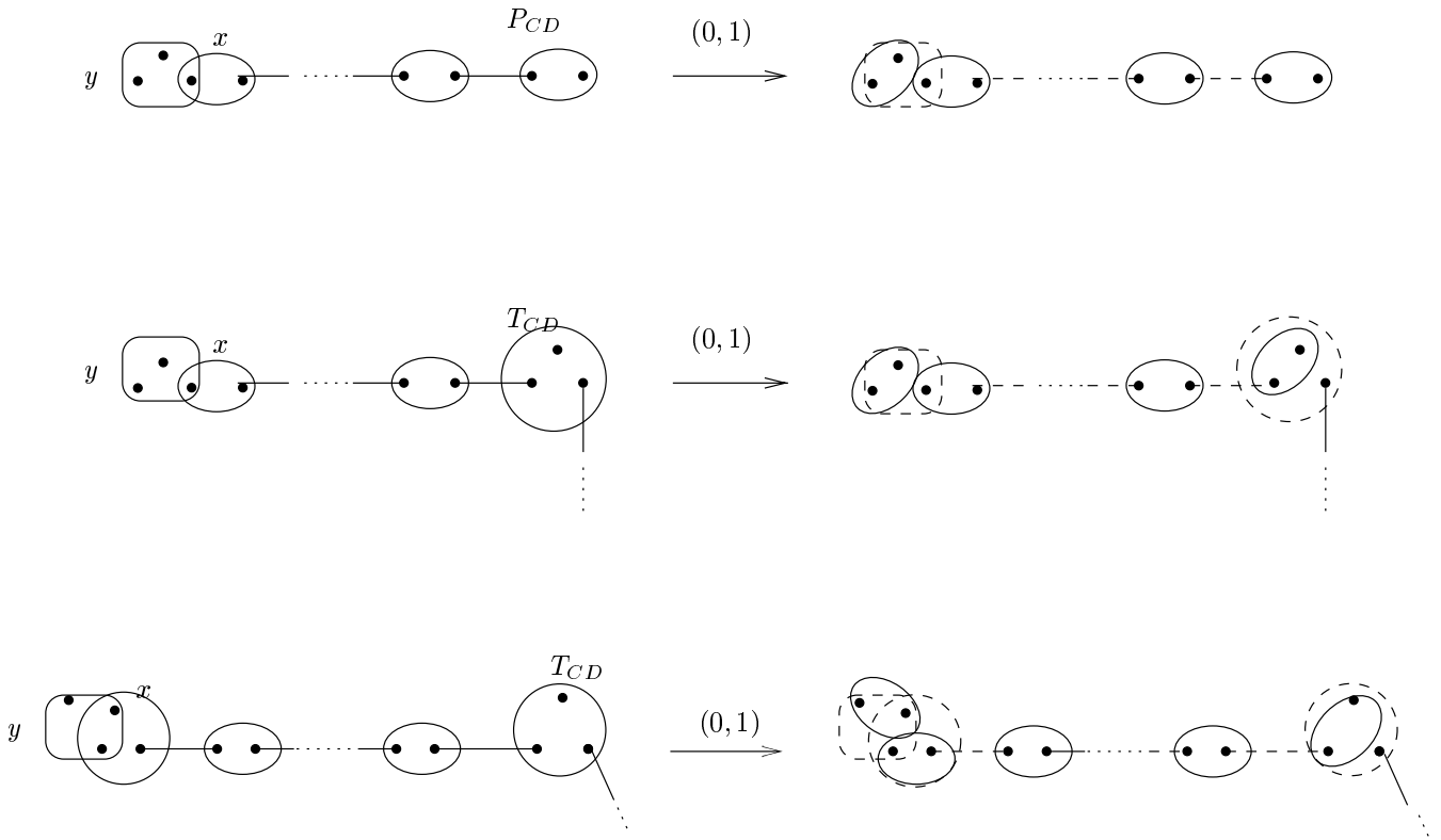
Figure 6: Examples for Lemma 3.6. In the above instances (0,1) semi-local improvement yields an improved solution.
