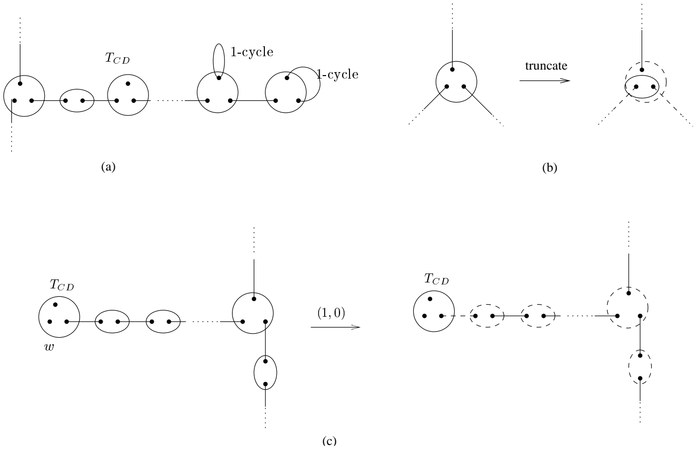
Figure 2: (a) Example of H . (b) Truncating a 3-set. (c) H can not have a T_{CD} covering two elements in D (Lemma 3.2).
