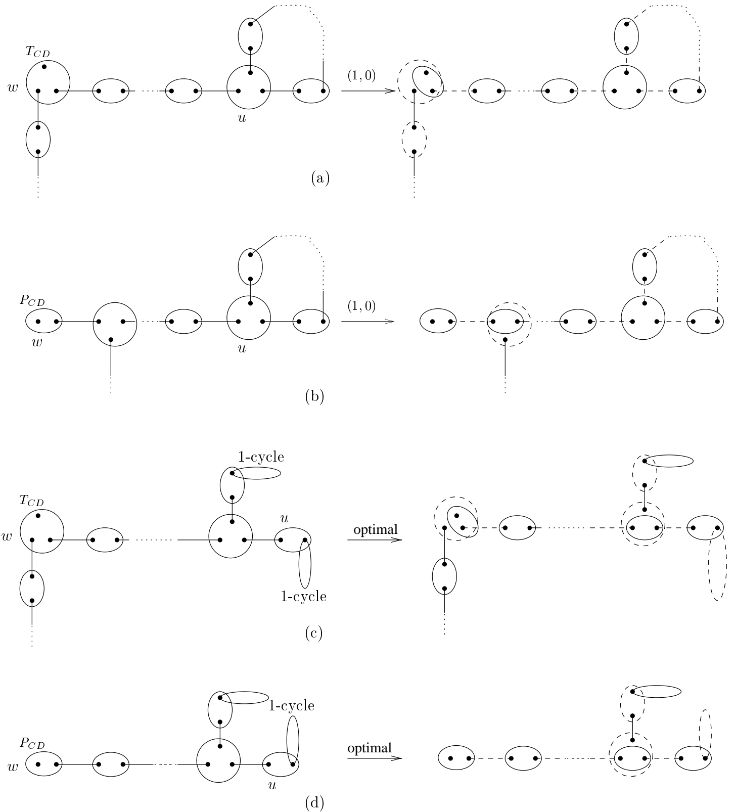
Figure 4: Examples for Lemma 3.4. In each of the following cases an improved partial cover (represented by figures on the right) contains the sets of OPT marked by solid boundaries and the sets of S corresponding to the solid edges. (a),(b) A (1, 0) optimization (inserting u ) gives us an improved solution. (c),(d) Our algorithm finds an optimal 2-cover. The figure on the left shows a sub-optimal 2-cover.
