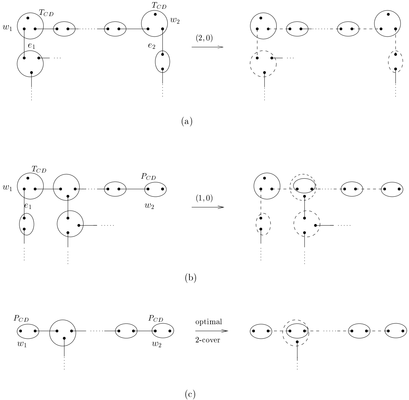
Figure 3: Examples for Lemma 3.3. In each of the following cases an improved partial cover (represented by figures on the right) contains the sets of OPT marked by solid boundaries and the sets of S corresponding to the solid edges. (a) Two T_{CD} sets in H lead to a (2,0) semi-local improvement. (b) A T_{CD} and P_{CD} in H leads to a (1,0) semi-local improvement. (c) Two P_{CD} sets in OPT is not possible as, w.l.o.g., our algorithm finds a solution maximizing the number of 2-sets belonging to OPT .
