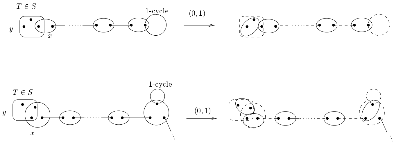
Figure 7: Examples for Lemma 3.8. In the above instances (0,1) semi-local improvement yields a cover whose size is same as before but has one less singleton.
