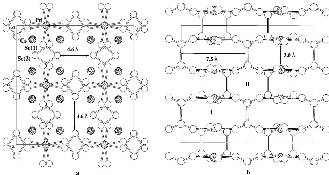
FIG. 2. Crystal structure of \text{Cs}_2\text{PdSe}_8 (1) projected along (a) the c -axis and (b) the a -axis. The shaded circles are Pd atoms, the open circles Se, and the doubly shaded circles Cs. The approximate dimensions of the open channels are indicated in the structure.
