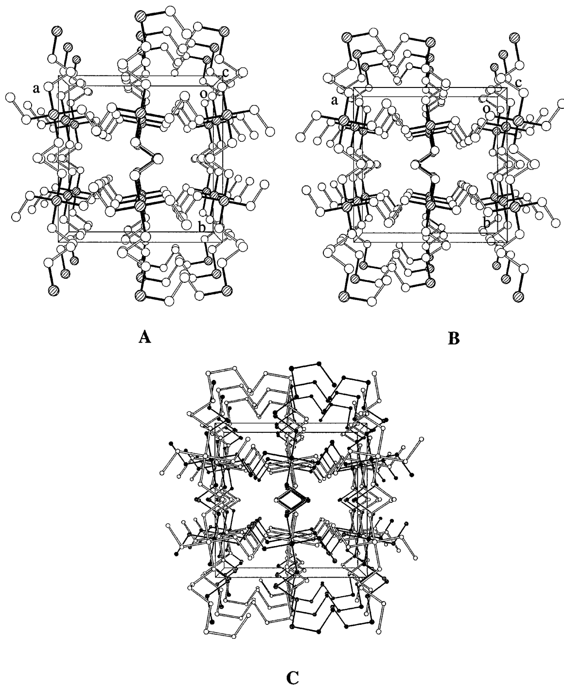
FIG. 3. Perspective views showing the two sub frameworks ( A and B ) and the overall three-dimensional \frac{2}{3}[\text{Pd}(\text{Se}_4)_2]^{2-} network upon insertion of the two sub-lattices ( C ). Framework A is shown in black in C . The approximate dimensions of the open channels in A and B are 6.4 \times 4.6 \text{ \AA} .
