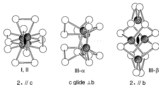
Figure 4. Views along the chain of [\text{In}_2\text{Te}_6]^{2-} for I , III-α , and III-β . The screw axis ( 2_1 ) in I , II , and III-β and the glide plane ( c -glide) in III-α are indicated in the figure. The cross-hatched circles are In atoms and the open circles Te.
