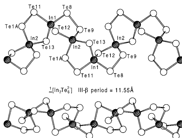
Figure 3. Two perpendicular views of the polymeric chain \alpha[\text{In}_2\text{Te}_6]^{2-} for III- \beta . The cross-hatched circles are In atoms and the open circles Te.
