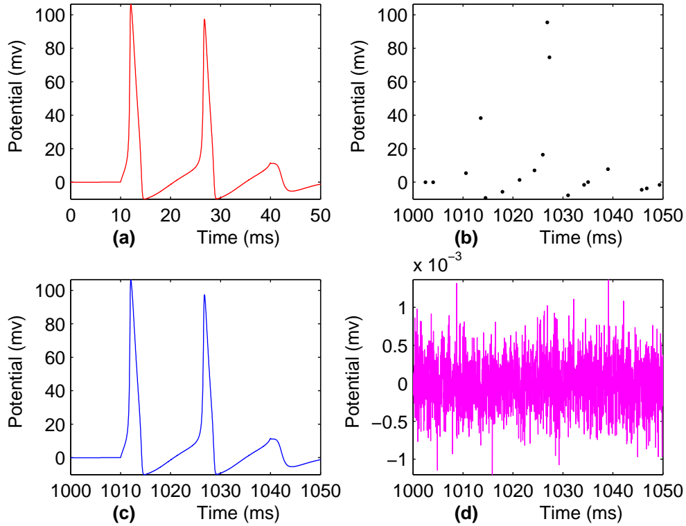
Fig. 1. (a) A numerical solution from the Hodgkin-Huxley equation (a standard model for electrical characteristics of neurons or cardiac myocytes) is taken as a signal \mathcal{S} . It should be noted that the signal is used in a general setting and is not meant to represent a specific biological situation. We suppose a correct response \mathcal{R} is essentially a duplicate of \mathcal{S} . (b) With N = 10^6 and \lambda_2 = 0.1105 , the link (u, v) ensures a probability \mu(\mathcal{A}_{\mathcal{S}}) = \exp\left(-\frac{N^2\lambda_2}{4}\right) = 0.005012 for \mathcal{S} to propagate, i. e., the link is an unreliable channel so that each h_{\mathcal{C}}((l + N)\tau) , l = 0 \dots, N_0 , is transformed with probability 0.005012. With no help from the internal noise, the response is disrupted: only a few elements of \mathcal{S} were transformed. It should be noted that the disrupted response is only for illustration. In a concrete biological network, such a disrupted response may well look differently, e. g., missing spikes in a train in a neural network. (c) With help of the internal noise, a correct response \mathcal{R} occurs. This response is \{h_{\mathcal{C}}((l + N)\tau) : l = 0, \dots, N_0\} obtained by the algorithm \mathcal{A}_h . (d) The result from the error checking in the algorithm \mathcal{A}_h shows the internal noise causes errors over the entire period. Since the internal noise is restricted at a low level, these errors are small. Importantly, through the 10^6 -dimensional product probability space induced by the internal noise, a correct response occurs shown in (c) as predicted by Theorem 1
